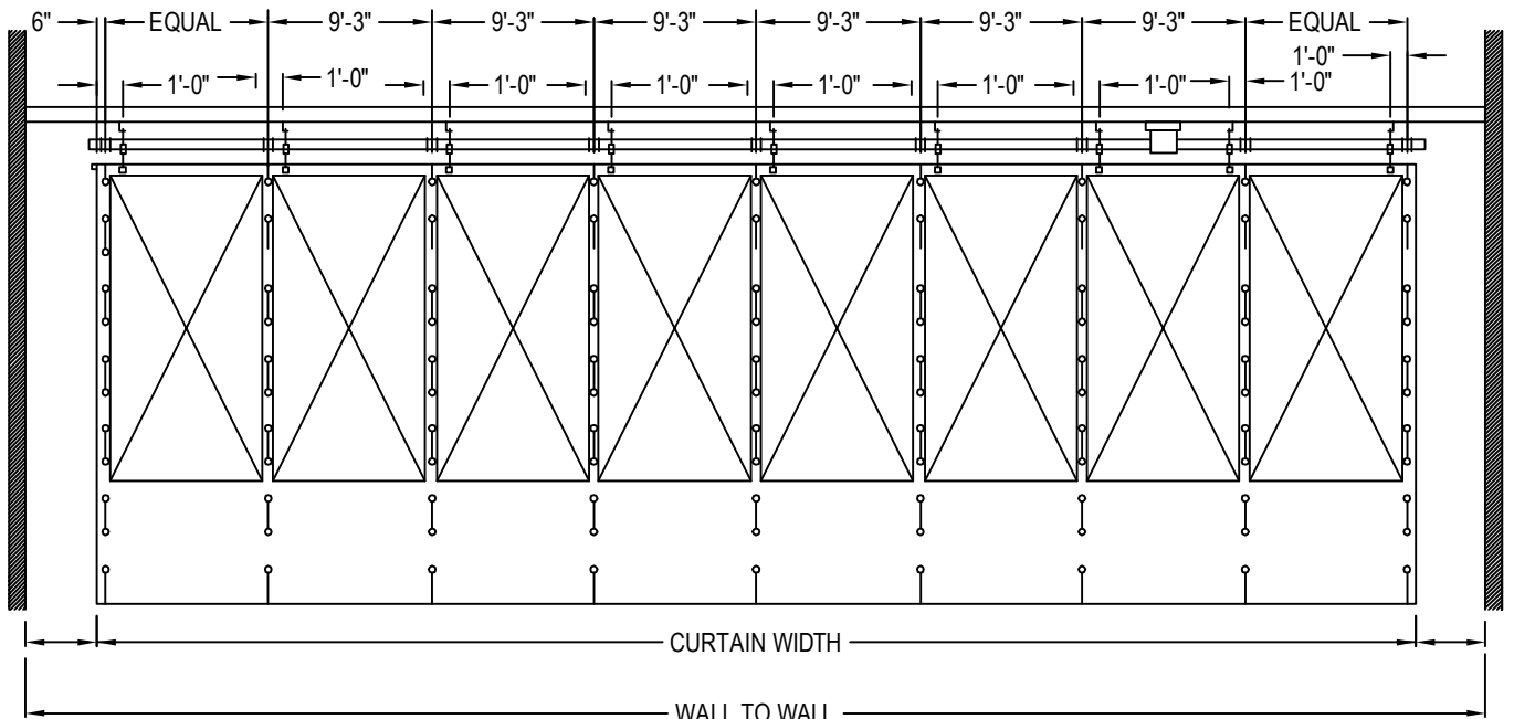
CURTAIN ELEVATION
