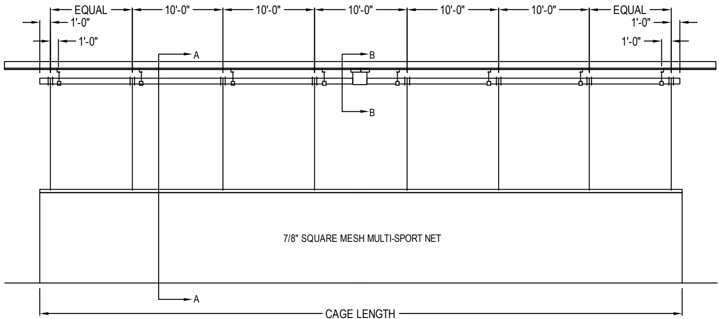
CURTAIN ELEVATION
