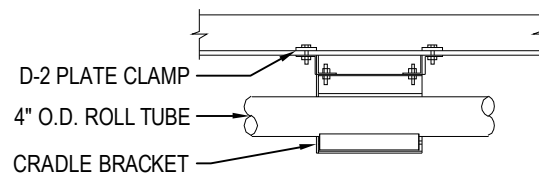
DRIVE TUBE LAYOUT
