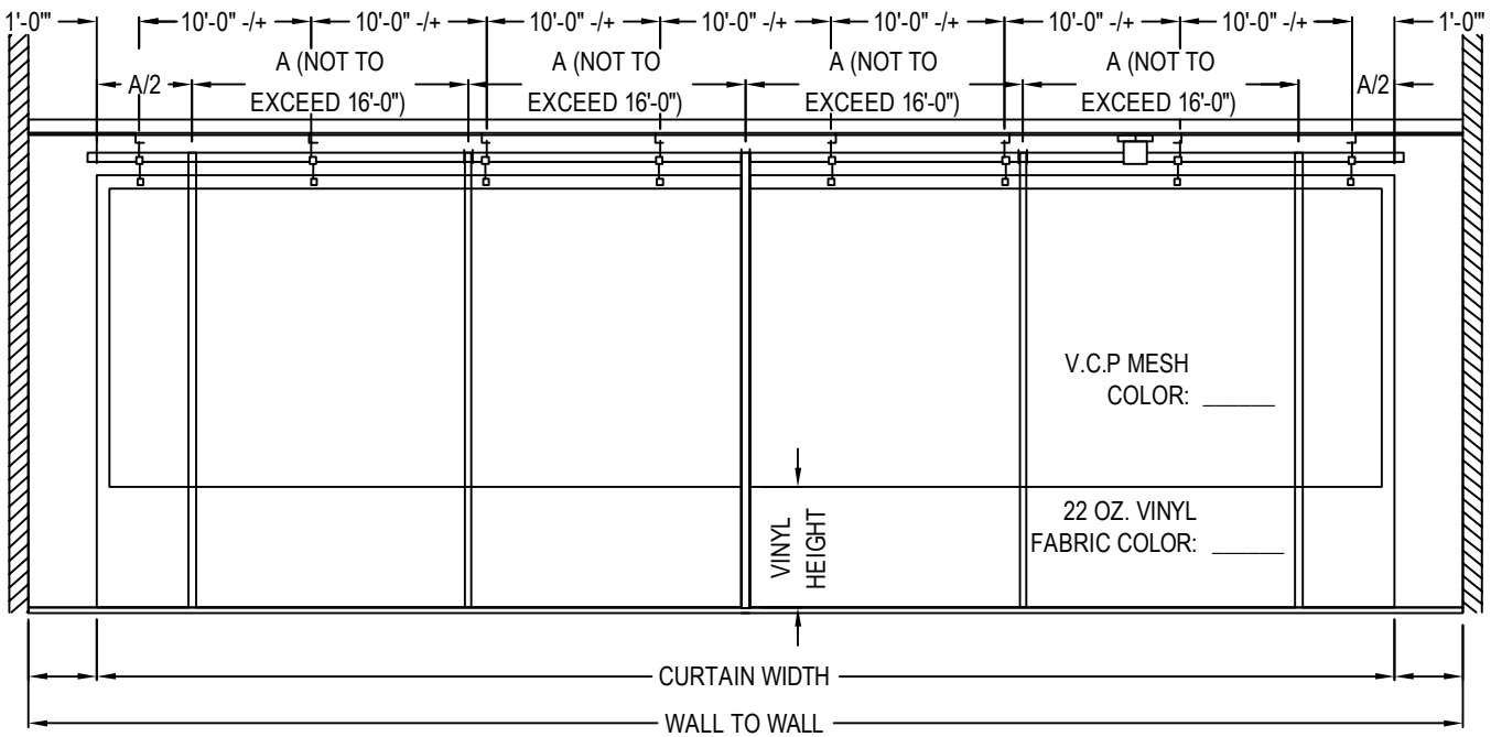
CURTAIN ELEVATION
