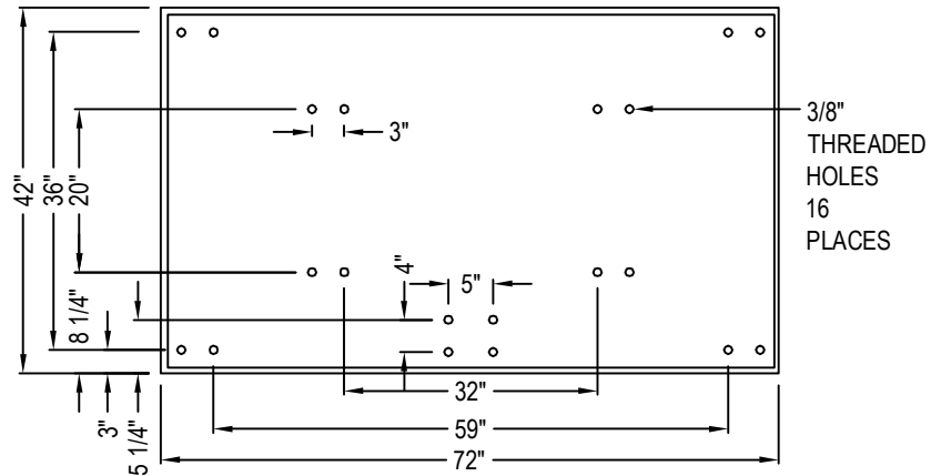
BACK VIEW
