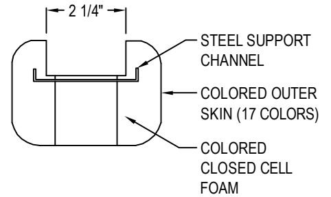
SECTION VIEW A-A BA68U PADDING (BOLT-ON)
