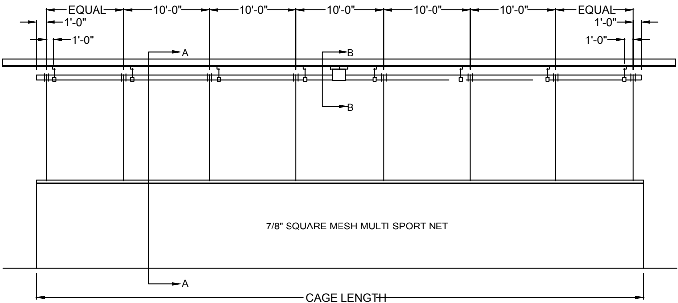
CURTAIN ELEVATION
