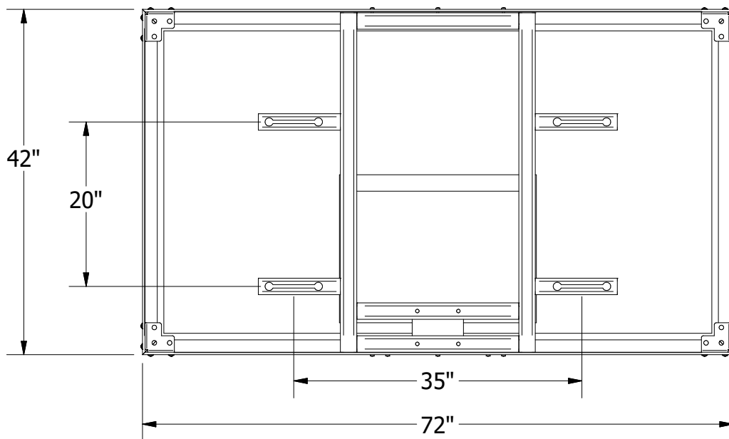
REAR
